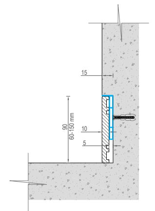
Плинтус со вставкой Plinth with insertion
