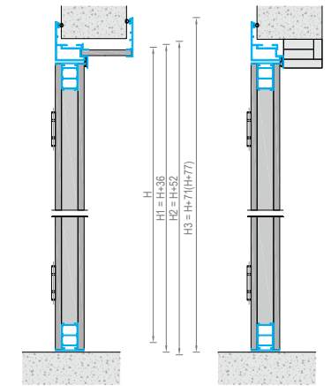
Монтаж с добором Installation with adjustment panel
