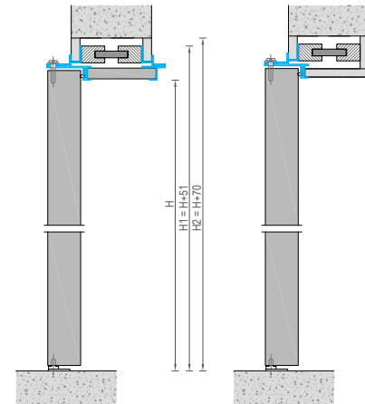
Монтаж с добором Installation with adjustment
